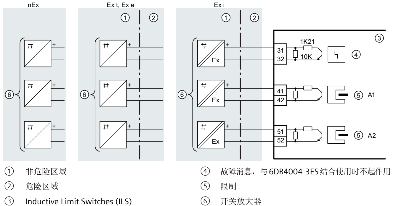
图 5-8 Inductive Limit Switches (ILS)
